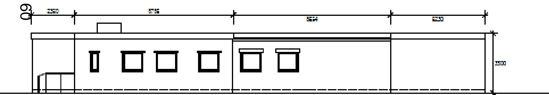
PROPOSED REAR ELEVATION SCALE 1/4"=1'-0"
