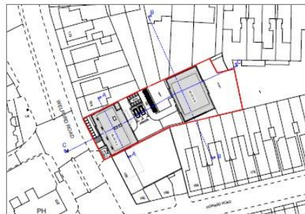
SITE PLAN KEY scale @ 1:500
